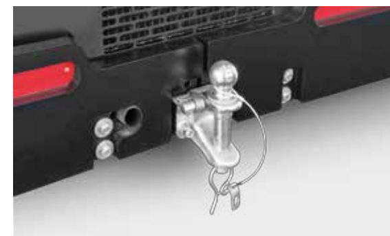
Trailer Hitch Homologated for use in road transit 115990101
